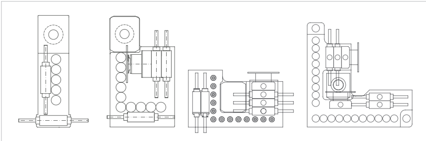
Available boring heads from 9 to 30 drill positions: BHZ 9 - BHZ 17 L - BHZ 24 L - BHZ 30 2L.
